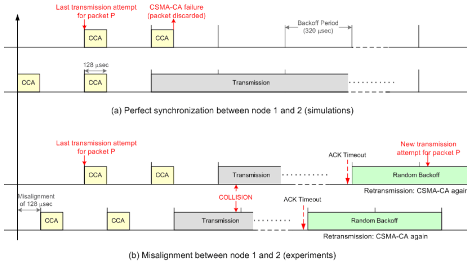
Figure 8. Effects of clock misalignment on packet transmissions.
