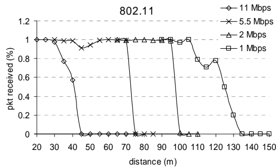
Figure 3. Packet reception probability for 802.11 nodes
