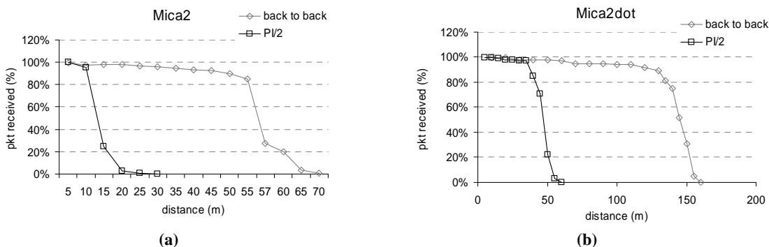
Figure 6. Communication distance as a function of antennas orientation for Mica2 (a) and Mica2dot (b)
