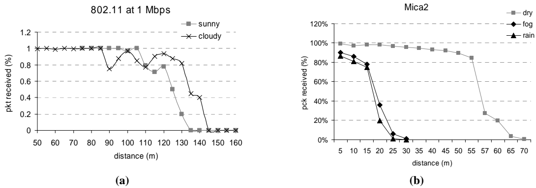
Figure 4. Communication distance in humid environments for 802.11 (a) and Motes (b) devices
