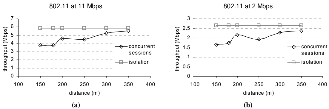
Figure 8. Sessions' throughput for 802.11 devices at 11 Mbps (a) and 2 Mbps (b)
