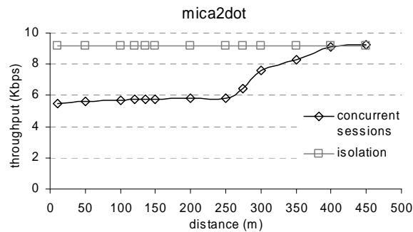
Figure 9. Sessions' throughput for Mica2dot Mote devices
