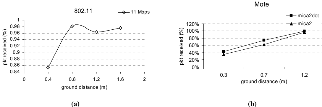
Figure 5. Impact of nodes height on the communication distance for 802.11 (a) and Motes (b) devices
