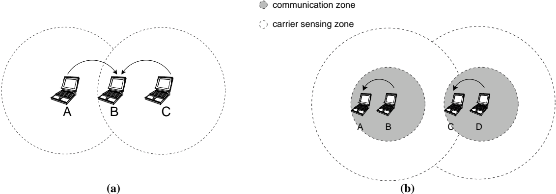
Figure 11. Traditional and novel formulation of the hidden node problem.
