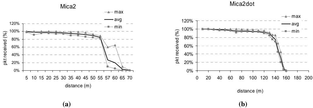
Figure 2. Packet reception probability for Mica2 (a) and Mica2dot (b)
