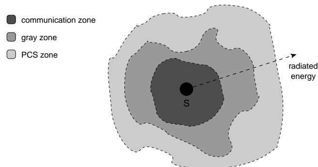
Figure 10. Unified channel model
