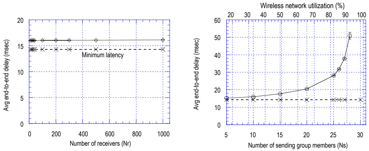
Figure 5. Latency with varying receivers (left) and with varying senders (right).
