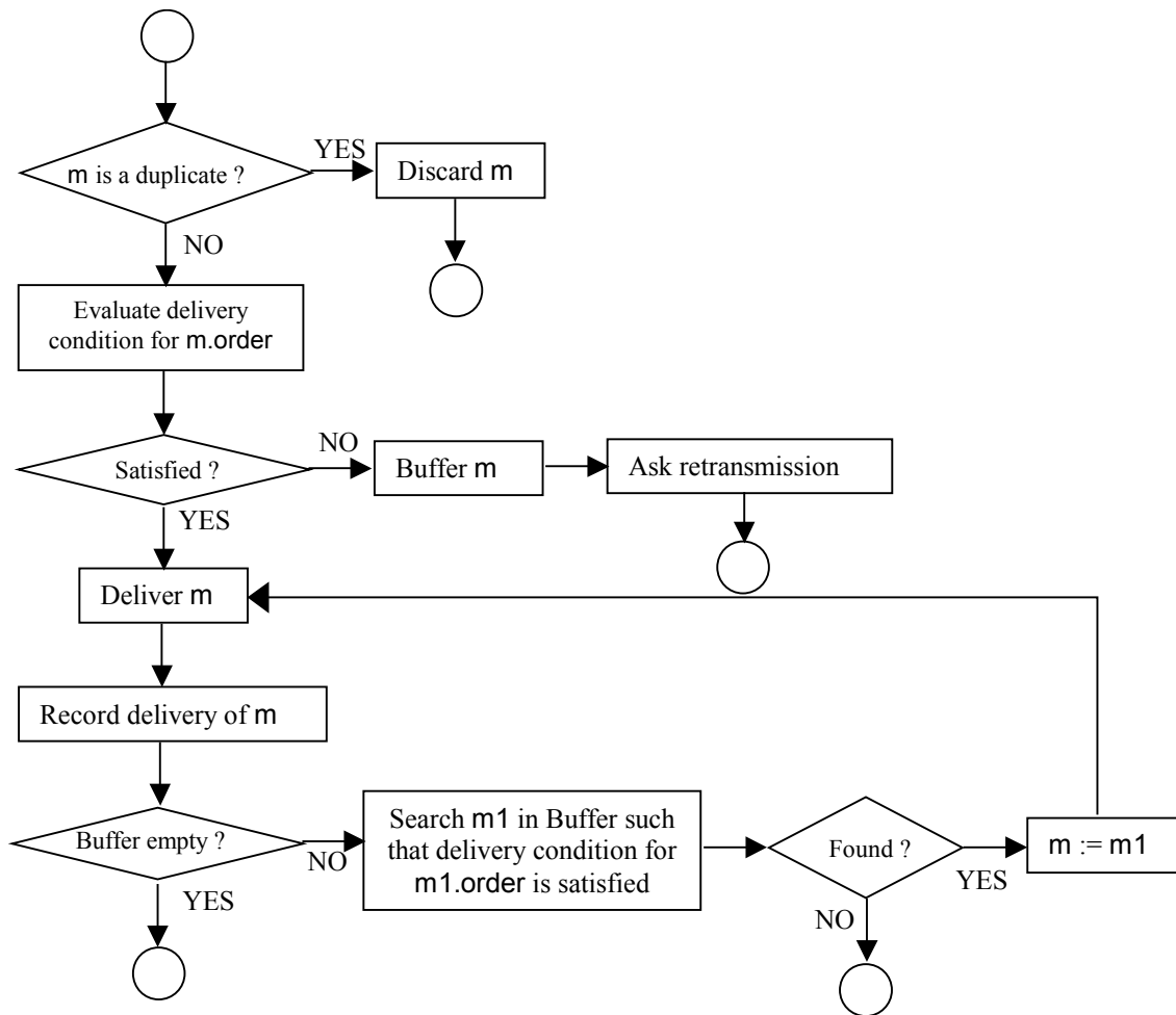
Figure 2. Group member's behavior while processing a NORMAL message.
