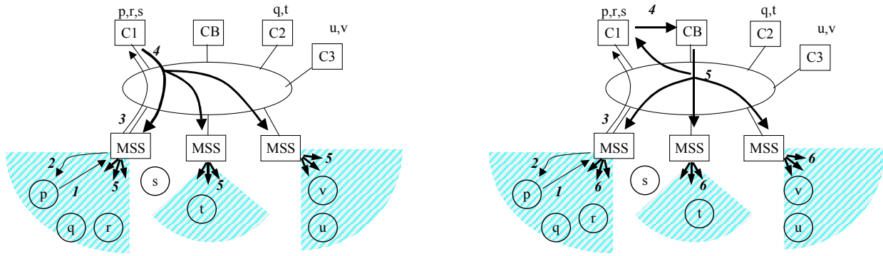
Figure 1. Message patterns for F-Cast(), C-Cast() (left) and for T-Cast() (right). Thin lines indicate NEW messages and acknowledgments, thick lines indicate NORMAL messages.
