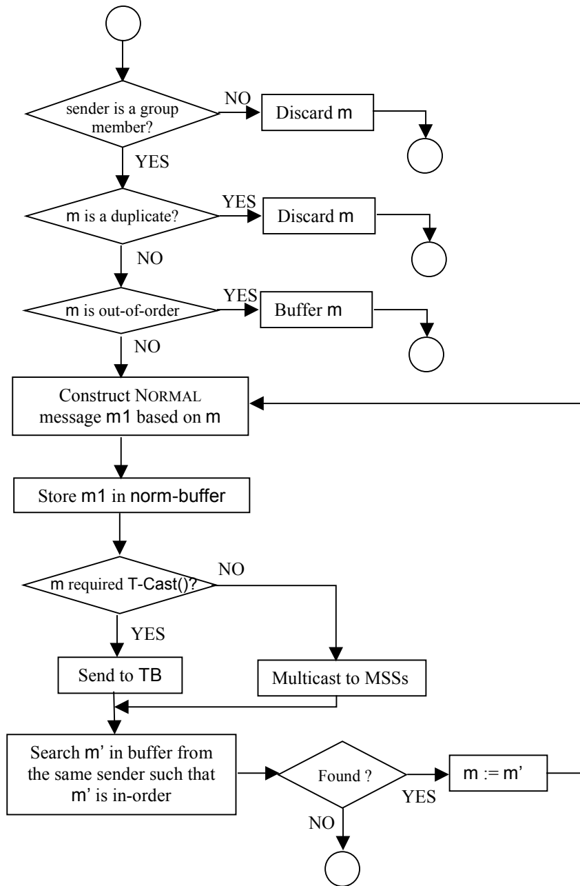
Figure 3. Coordinator's behavior while processing a NEW message.
