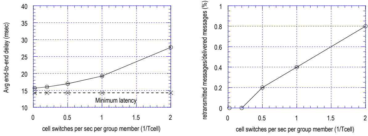
Figure 6. Average latency (left) and percentage of retransmitted messages (right) vs. host mobility.
