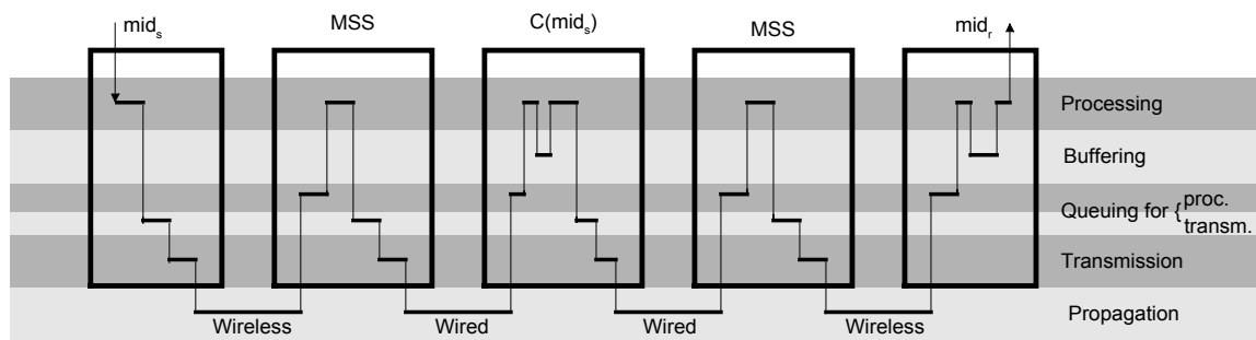
Figure 4. Delays experienced by a message in case no message loss occurs (relative lengths of time intervals do not reflect their actual values).
