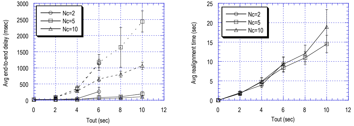
Figure 7. Average latency (left) and average re-alignment delay (right) vs. out-of-coverage permanency time ( T_{out} ) for disconnecting (dashed lines) and non-disconnecting (continuous lines) members. N_c does not include the boss.
